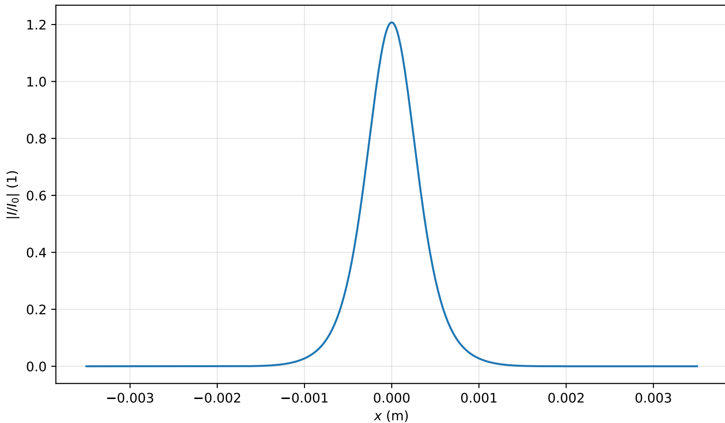
Intensity profile I(x, y = 0, z = 1.353m)/I_0 , P_{in}=0.7P_{cr} , artificial time
